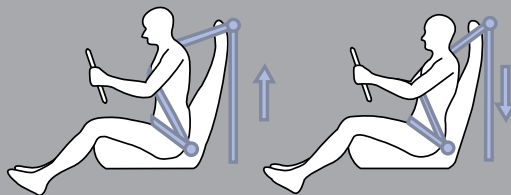
Front Seat Belts Pretensioner with Load Limiter
